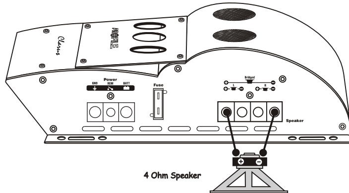
TWO CHANNEL BRIDGED SPEAKER CONNECTIONS
